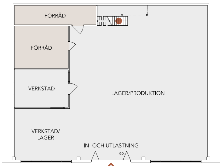
BOTTENPLAN
